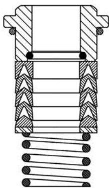
LIVE-LOADED PTFE - V-RING (STANDARD)
