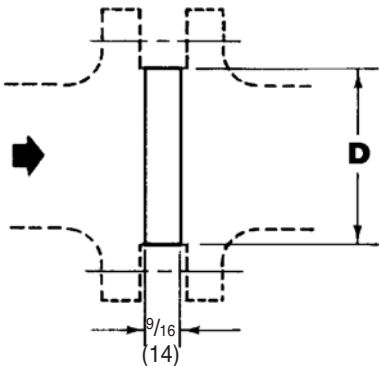
ANSI 250, 300 & 600 FLANGED
