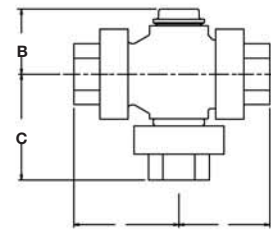
K3, K7 1/2" - 2"
