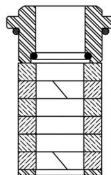
HIGH TEMPERATURE LAMINATED GRAPHITE (OPTIONAL)
